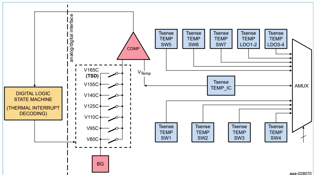
Figure 32. Thermal monitoring architecture
