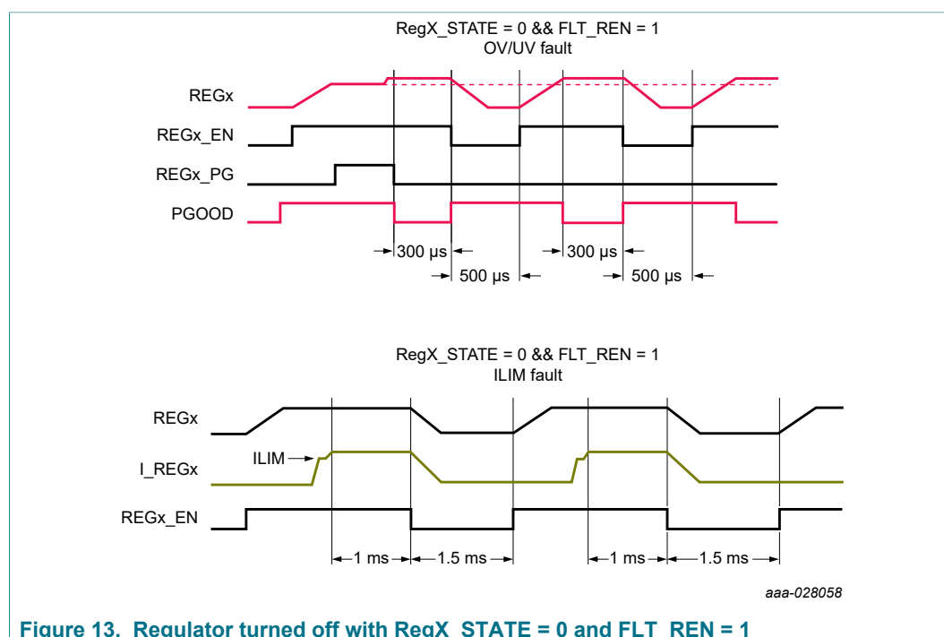
Figure 13. Regulator turned off with \text{RegX\_STATE} = 0 and \text{FLT\_REN} = 1
