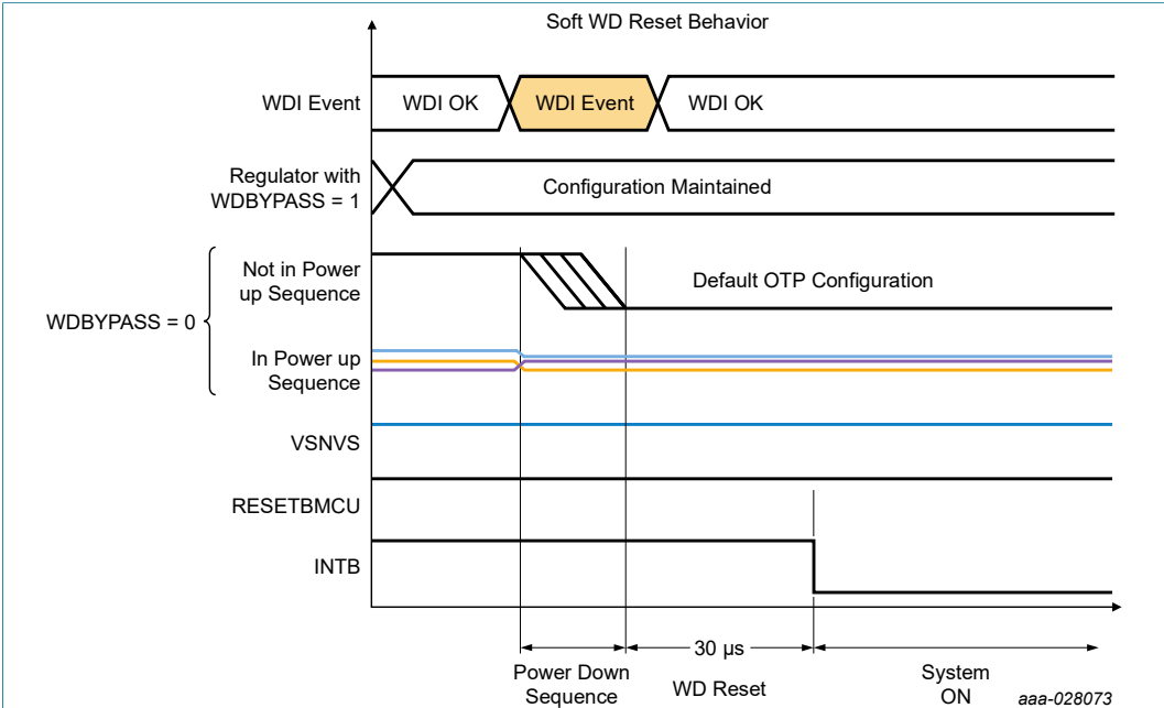
Figure 35. Soft WD reset behavior
