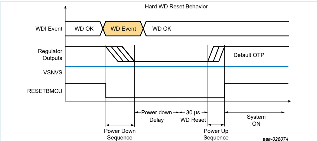
Figure 36. Hard WD reset behavior
