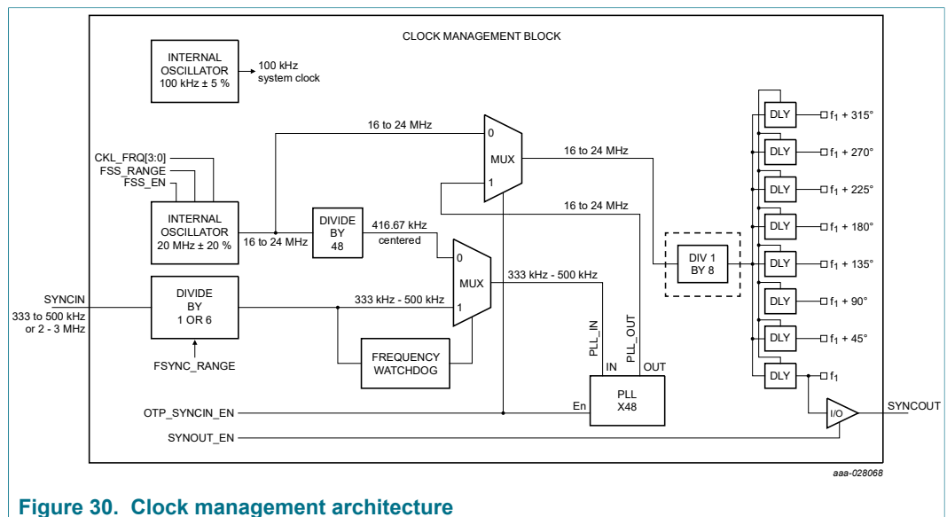
Figure 30. Clock management architecture
