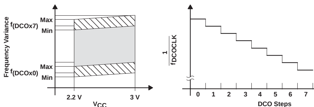
Figure 4. DCO Characteristics
