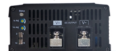
DC output side
