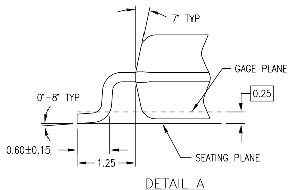
Figure 13. 14-Lead Small Outline Package (SOP), EIAJ TYPE II, 5.3mm Wide
