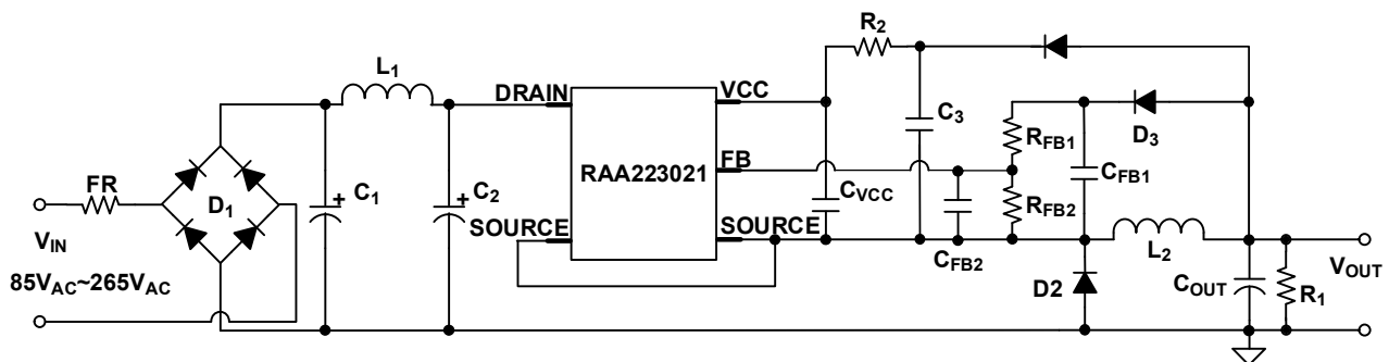
Figure 29. RAA223021 Buck with 5V Output
