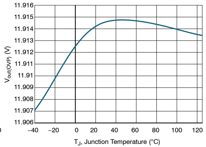
Figure 51. V out(OVP) vs. Temperature
