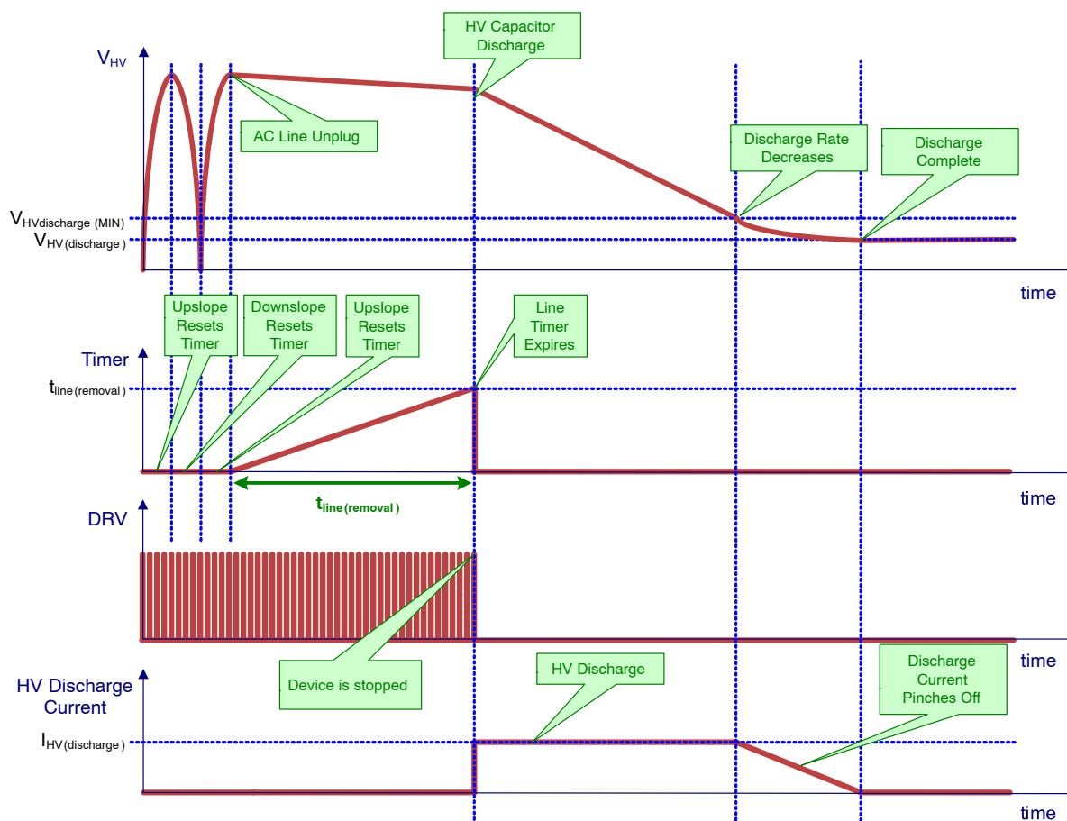
Figure 26. HV Discharge Timing
