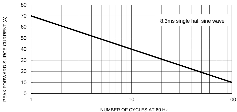
Fig.5 Maximum Non-Repetitive Forward Surge Current
