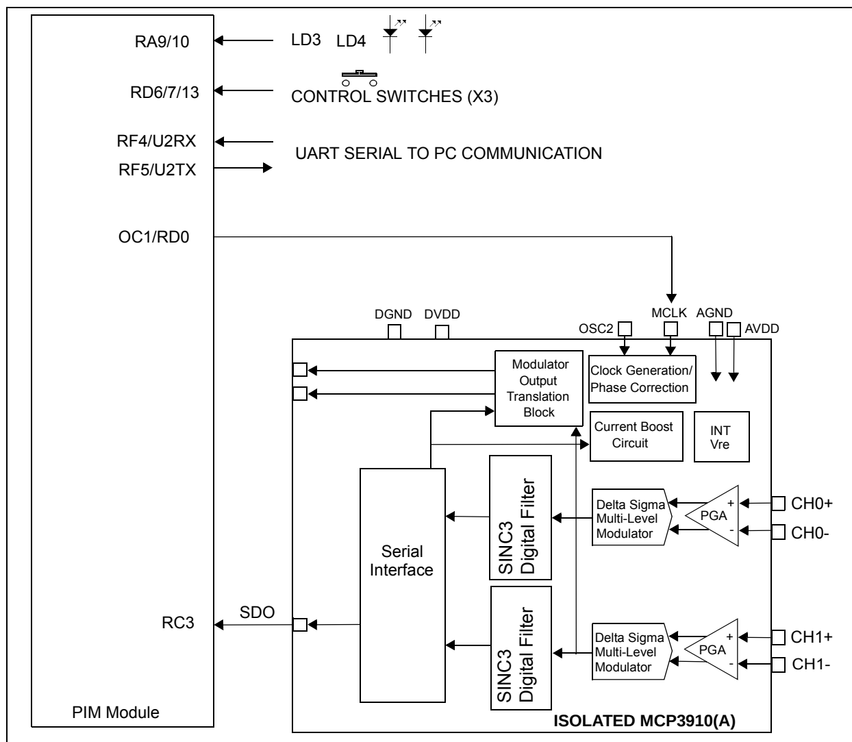
FIGURE 1-9: Digital Connection Overview PIM/MCP3910(A) Isolated Connections.
