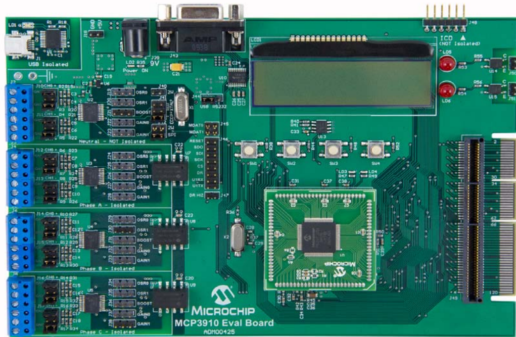
FIGURE 1-2: MCP3910 Evaluation Board.
