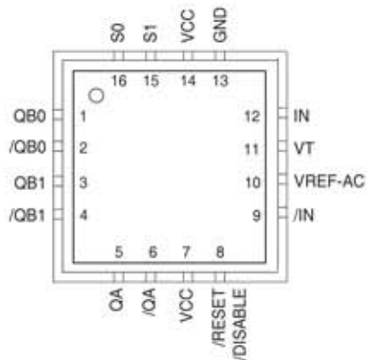
16-Pin QFN
