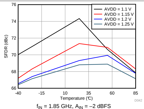
Figure 44. Spurious-Free Dynamic Range vs AVDD Supply and Temperature
