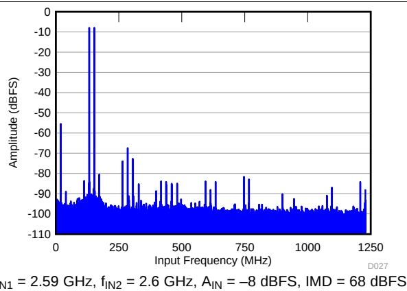
Figure 27. FFT for Two-Tone Input Signal (–8 dBFS)
