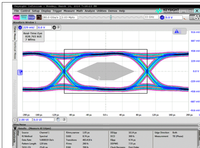
Figure 122. Data Eye at 5 Gbps
