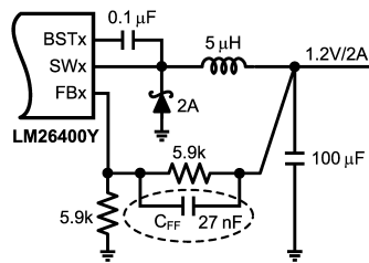
Figure 31. Adding a C_{FF} Capacitor
