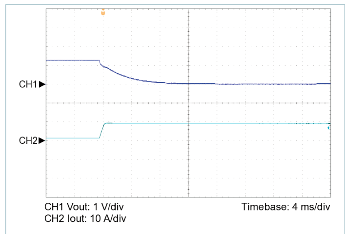
Figure 8 — 10% to 100% load transient response, V_{IN} = 24\text{ V} , nominal trim, C_{OUT\_EXT} = 250\text{ }\mu\text{F}
