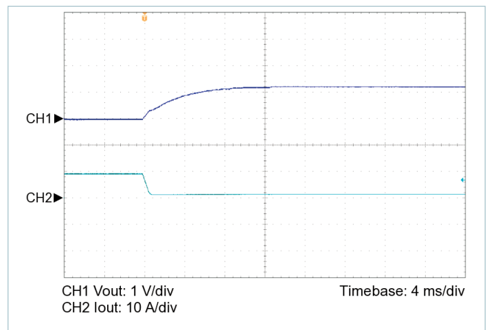
Figure 7 — 100% to 10% load transient response, V_{IN} = 24\text{ V} , nominal trim, C_{OUT\_EXT} = 250\text{ }\mu\text{F}
