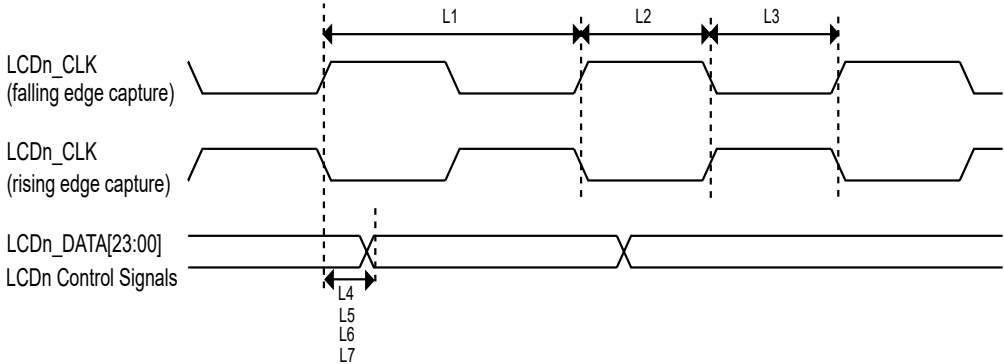
Figure 29. LCD timing
