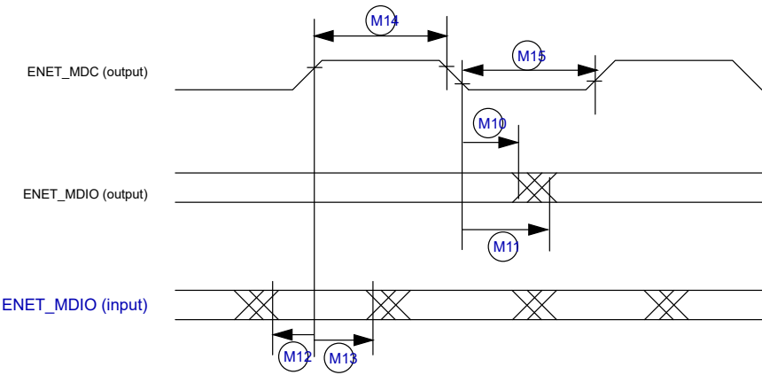
Figure 49. MII serial management channel timing diagram
