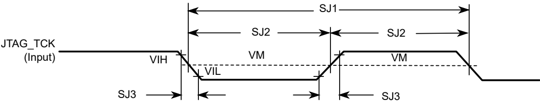
Figure 11. Test clock input timing diagram
