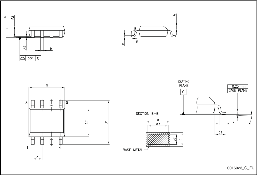
Figure 13. SO-8 package dimensions
