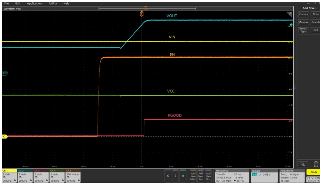
Figure 21 Startup into pre-bias (Ch1:PV IN , Ch2: V OUT , Ch3: PGood, Ch4:V CC , Ch5: Enable)
