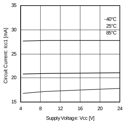
Fig.7 Supply current 1 (forward) (BA6285AFP-Y)
