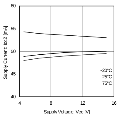
Fig.4 Supply current 2 (brake) (BA6287F)
