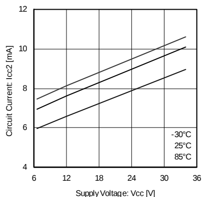
Fig.10 Supply current 2 (brake) (BA6920FP-Y)
