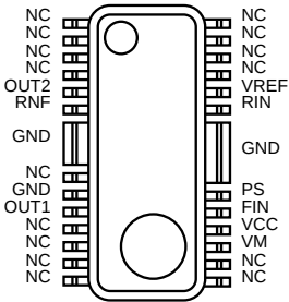
Fig.34 BA6920FP-Y (HSOP25)
