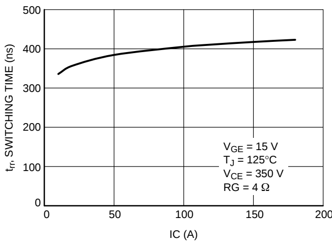
Figure 33. Half Bridge Forward Diode Typical Reverse Recovery Time vs. I_C
