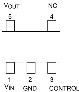
SMV(SOT-25)(SC-74A)
