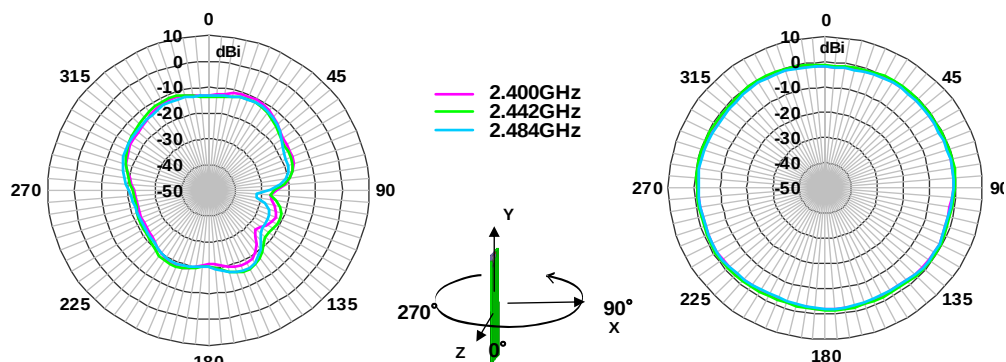
Horizontal Polarization
