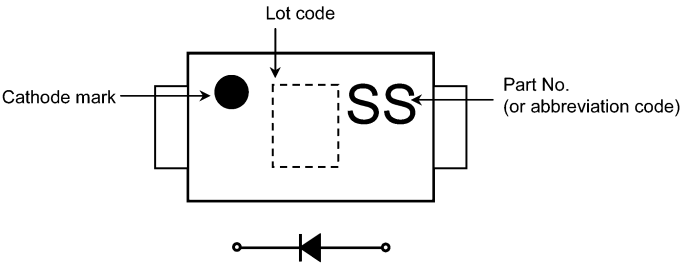
Fig. 7.1 Marking
