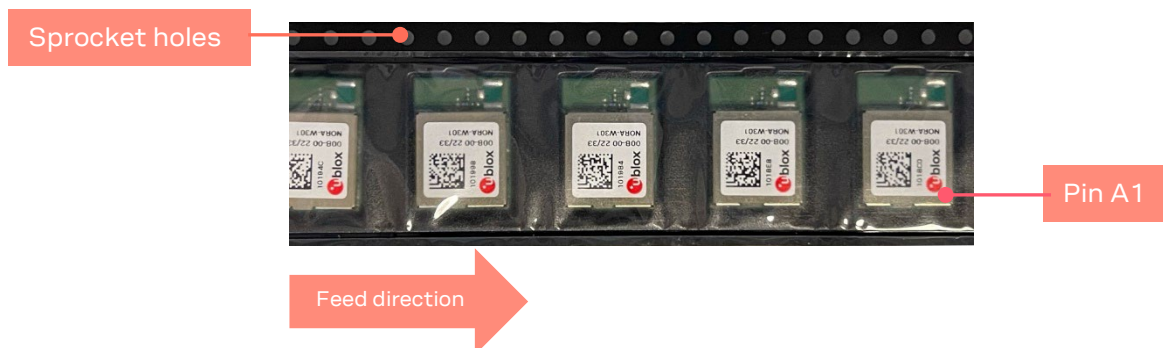
Figure 7: NORA-W361 module on tape orientation
