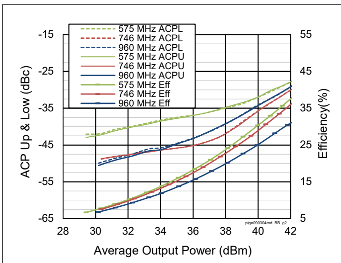
Figure 10. Single-carrier WCDMA 3GPP Drive-up
