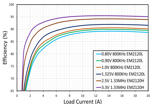
Efficiency, V_{IN} = 5V
