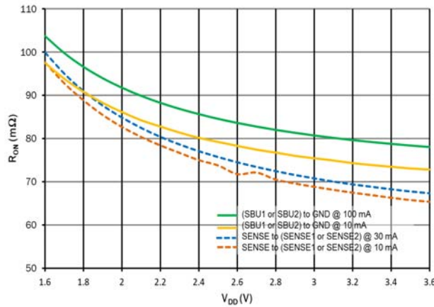
Figure 6. R_{ON} (GND/SENSE @ I_I = 1 mA)
