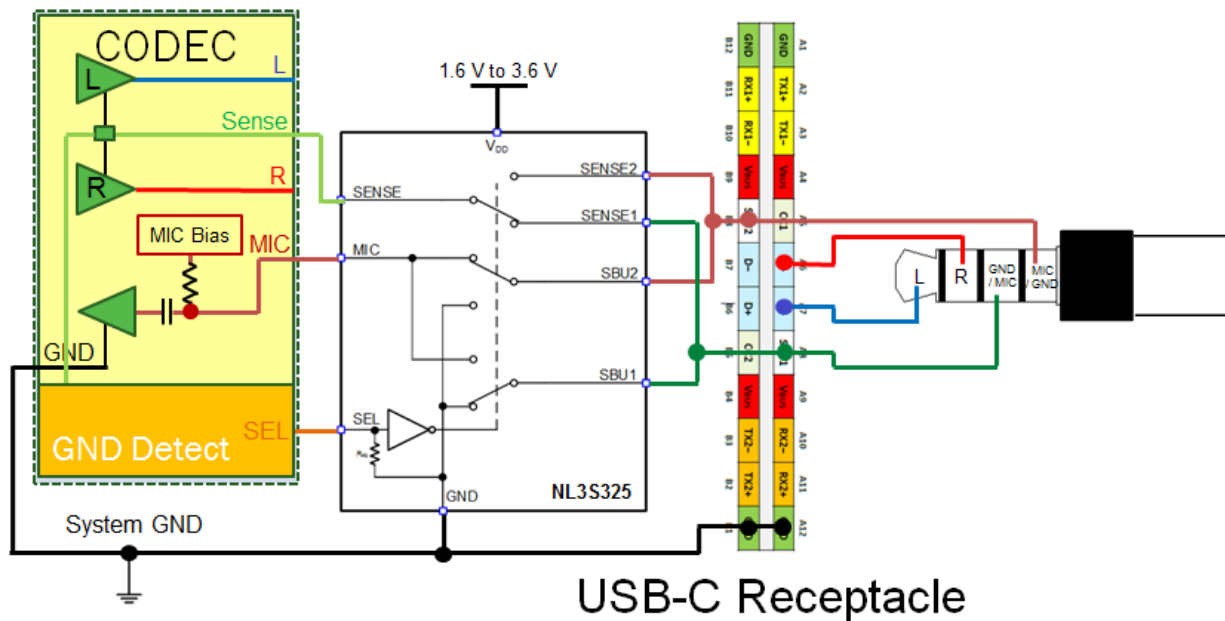
Figure 3. Typical Application
