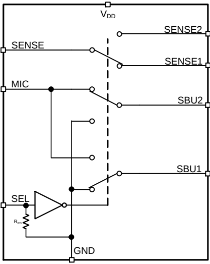
Figure 1. Block Diagram
