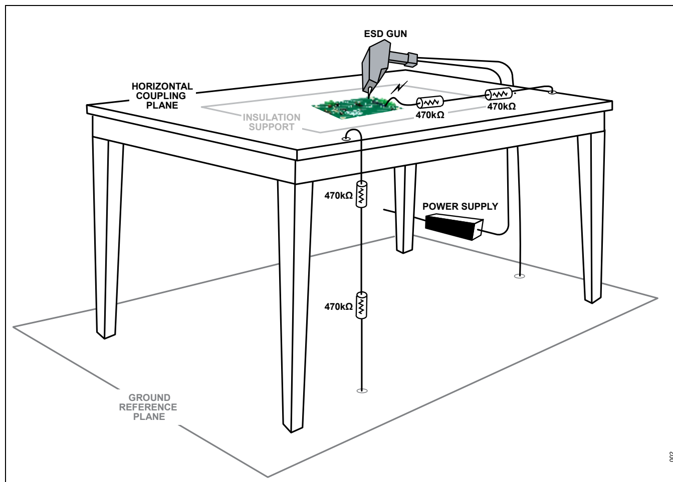
Figure 1. IEC 61000-4-2 ESD Test Setup
