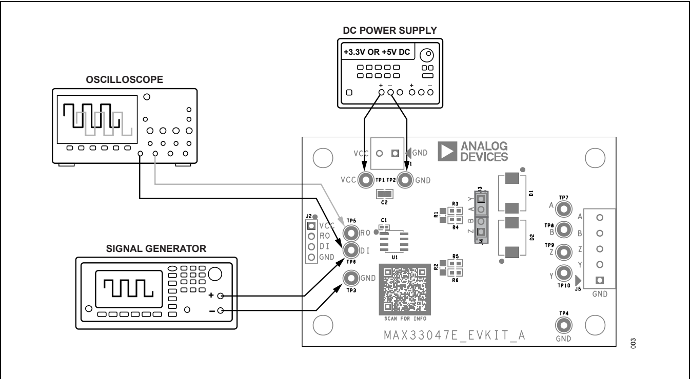
Figure 2. Connection Diagram
