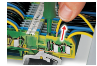
CAGE CLAMP® connection Removing a solid conductor.
