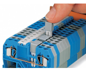
Commoning using an adjacent jumper. Push jumper down until fully inserted!
