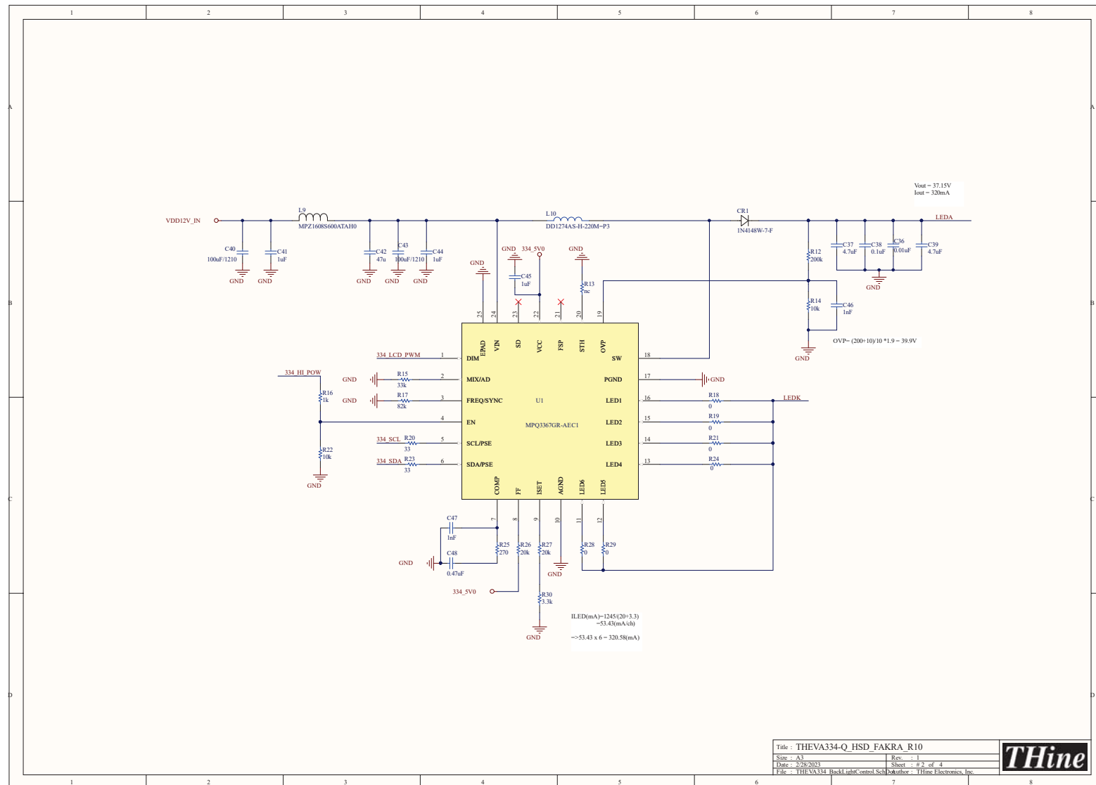
Figure 15. THEVA334-Q_HSD_FAKRA Schematics -2/4
