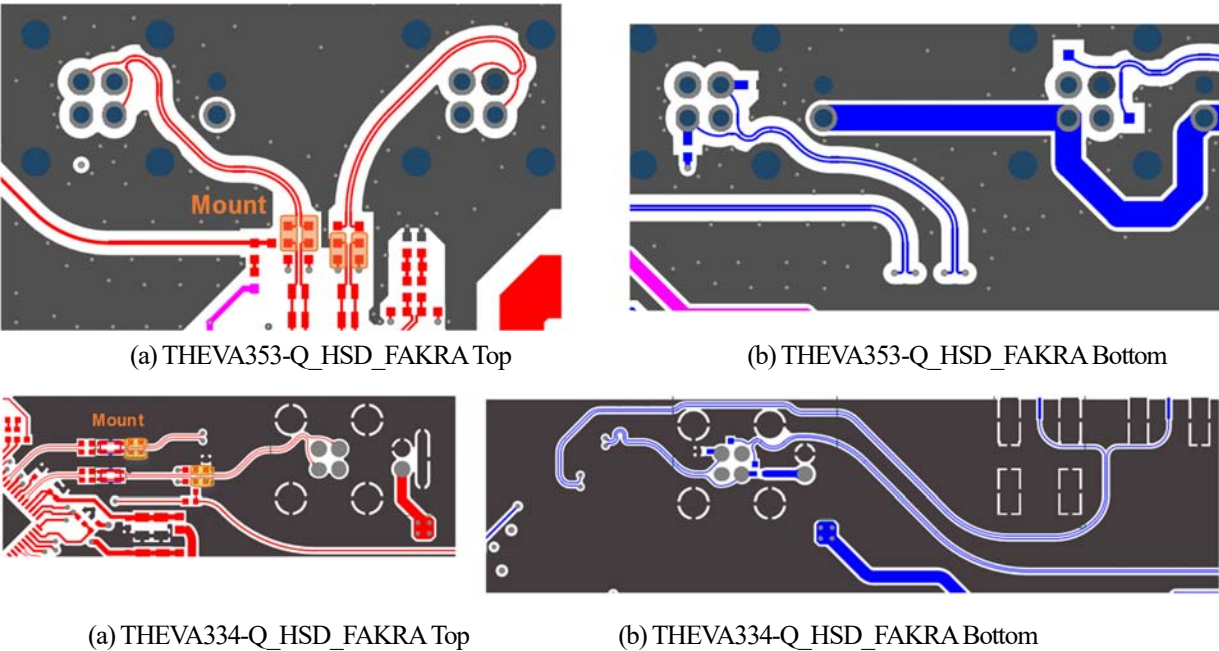
Figure 2. Mount/Unmount Components Locations for 6pin-HSD Cable
