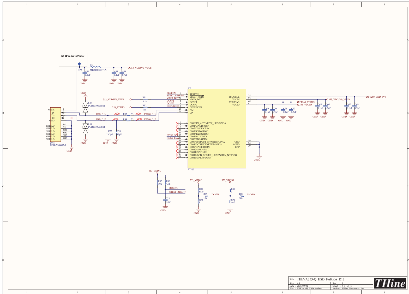
Figure 11. THEVA353-Q_HSD_FAKRA Schematics -3/5
