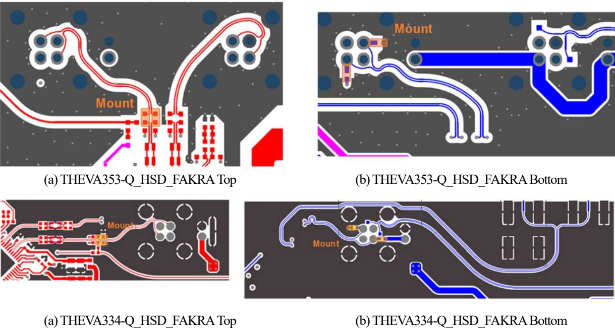
Figure 3. Component Locations for V-by-One®HSII Single Link and 12V Power/GND with 4pin-HSD Cable
