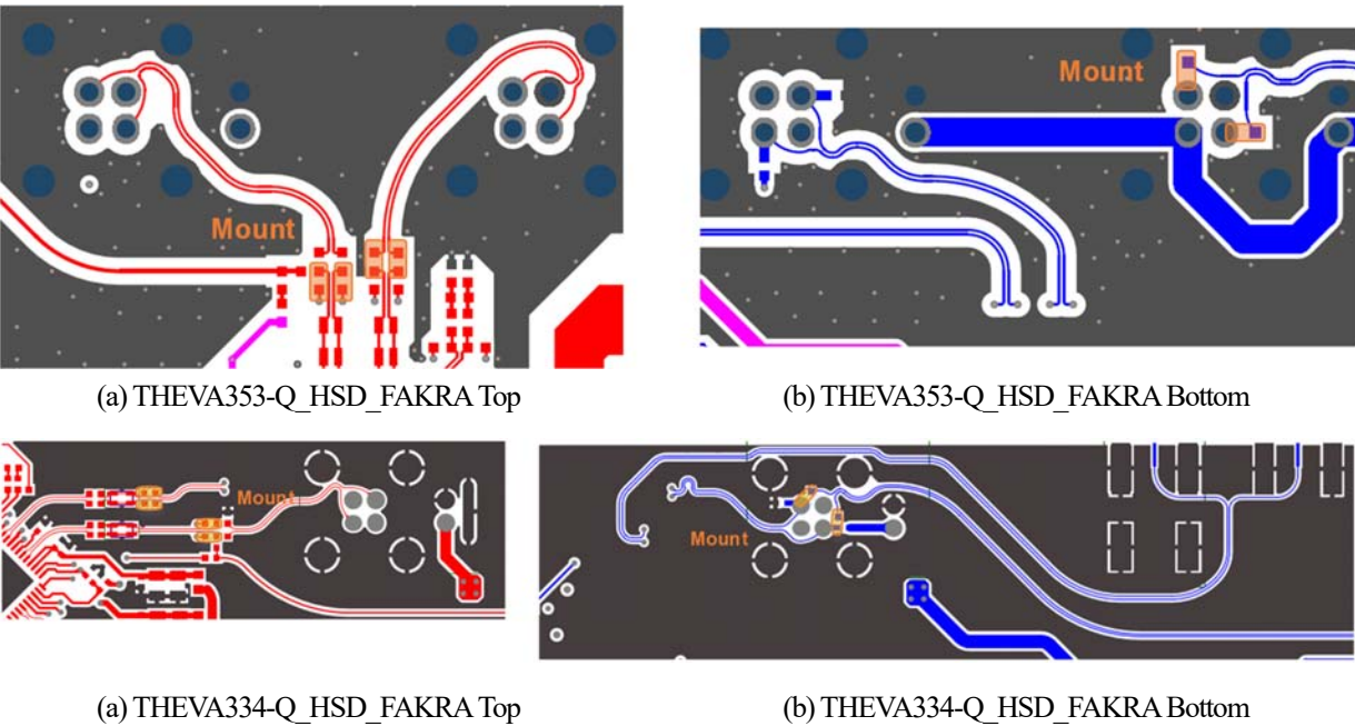
Figure 5. Component Locations for V-by-One®HSII Dual Link with SMA Cables
