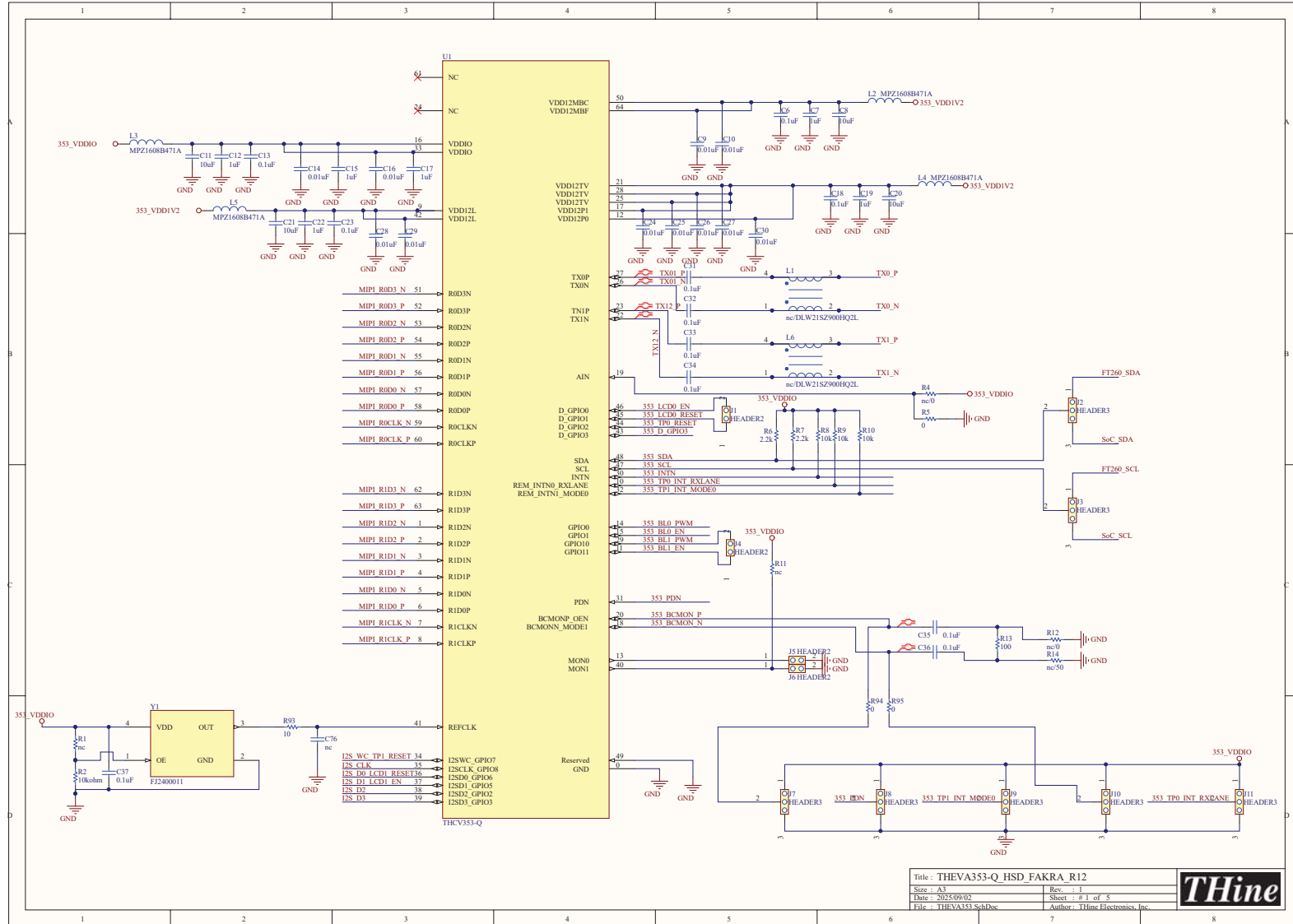
Figure 9. THEVA353-Q_HSD_FAKRA Schematics -1/5
