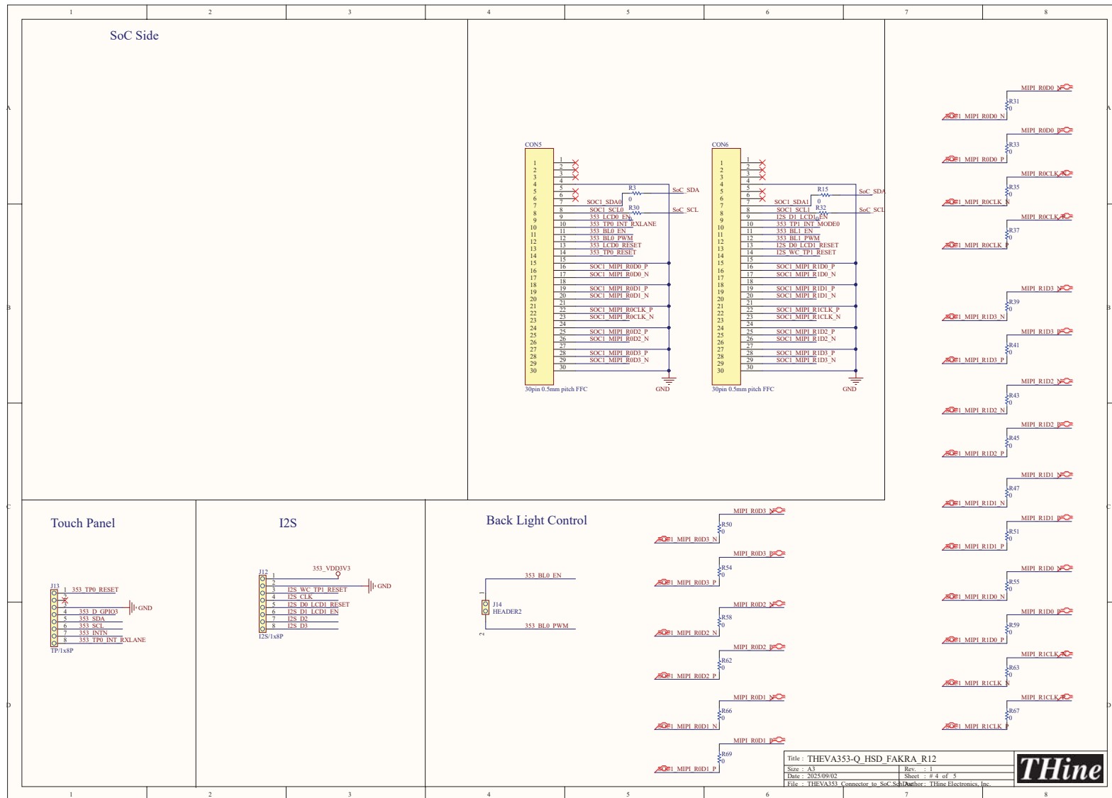
Figure 12. THEVA353-Q_HSD_FAKRA Schematics -4/5
