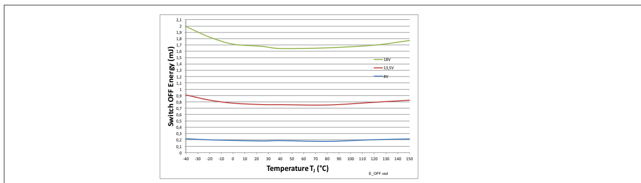
Figure 41 Switch OFF Energy E_{OFF} = f(T_J; V_G) , R_L = 2 \Omega
