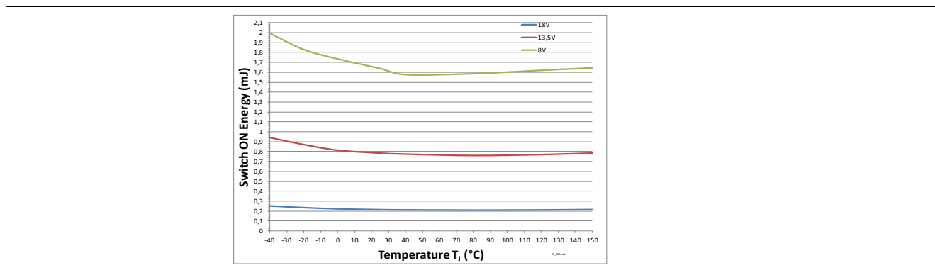
Figure 40 Switch ON Energy E_{ON} = f(T_J; V_G) , R_L = 2 \Omega
