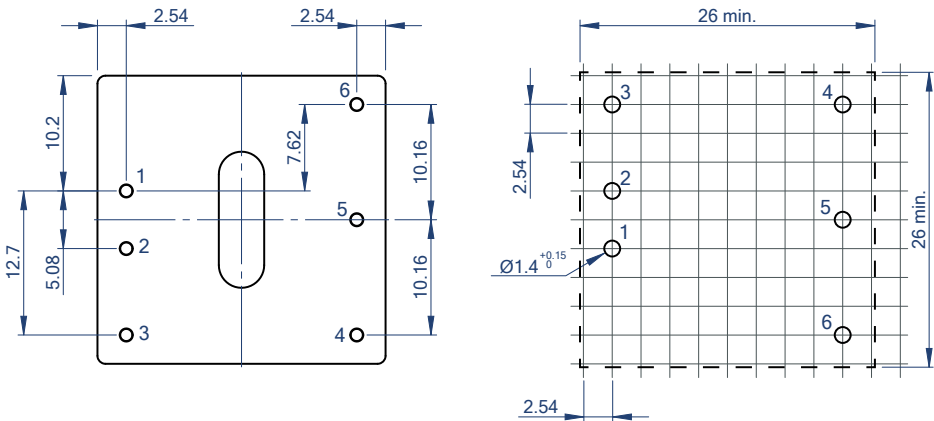
Recommended Footprint Details
