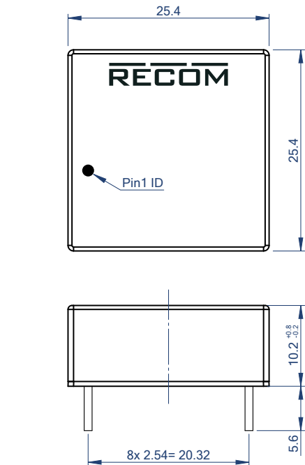
Dimension Drawing (mm)
