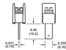
09 0.250" QC short
