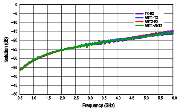
Figure 4. Isolation vs Frequency, ANT2-TX/ANT1-RX Insertion Loss Mode
