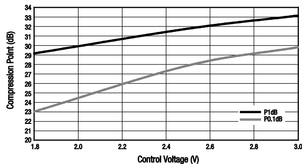
Figure 8. P1dB and P0.1dB vs Control Voltage @ 5.5 GHz
