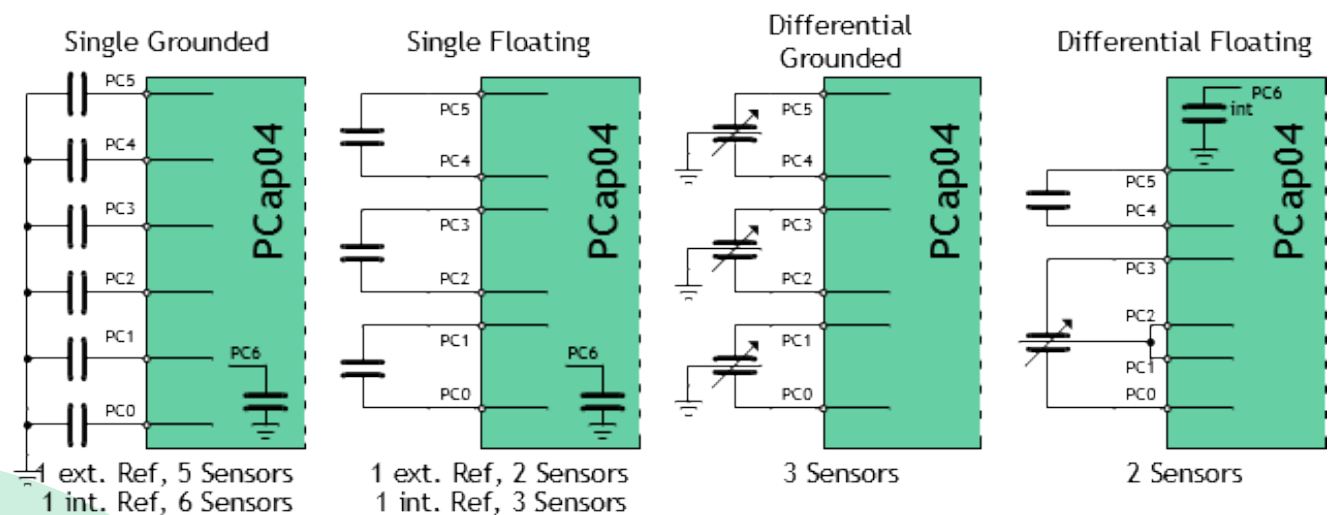
Figure 5: Connecting sensors
