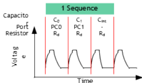
Figure 10: Sequence Grounded
