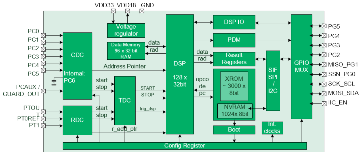
Figure 1: Functional Blocks
