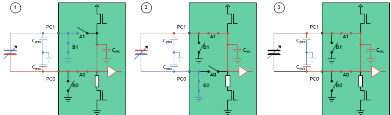
Figure 16: External Compensation
