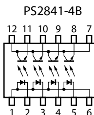
PIN CONNECTIONS (Top View)
