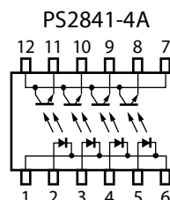
PIN CONNECTIONS (Top View)
