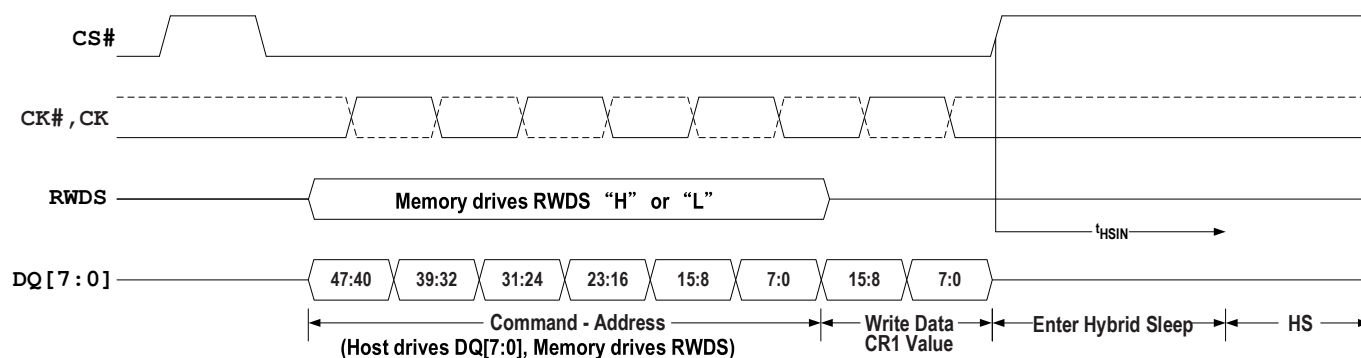
Figure 14 - Enter Hybrid Sleep Transaction
