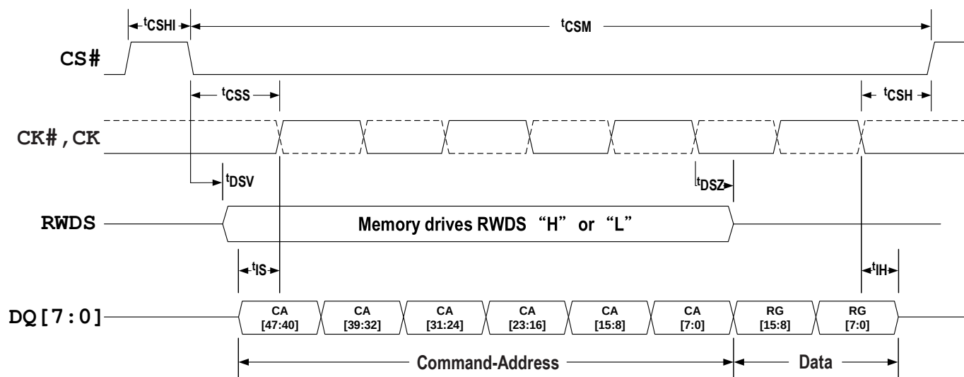
Figure 32 - Write Operation without Initial Latency (Register Write)
