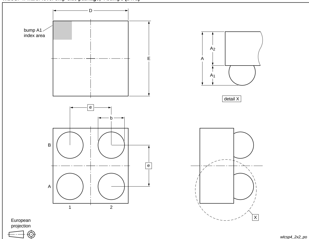
Fig 16. Package outline IP4369CX4 (WLCSP4)
