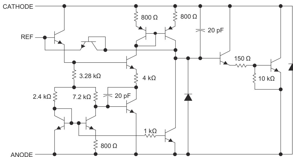
Figure 9-2. Detailed Schematic
