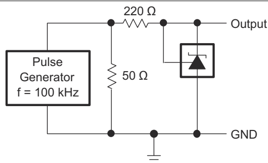
Figure 7-15. Test Circuit for Pulse Response
