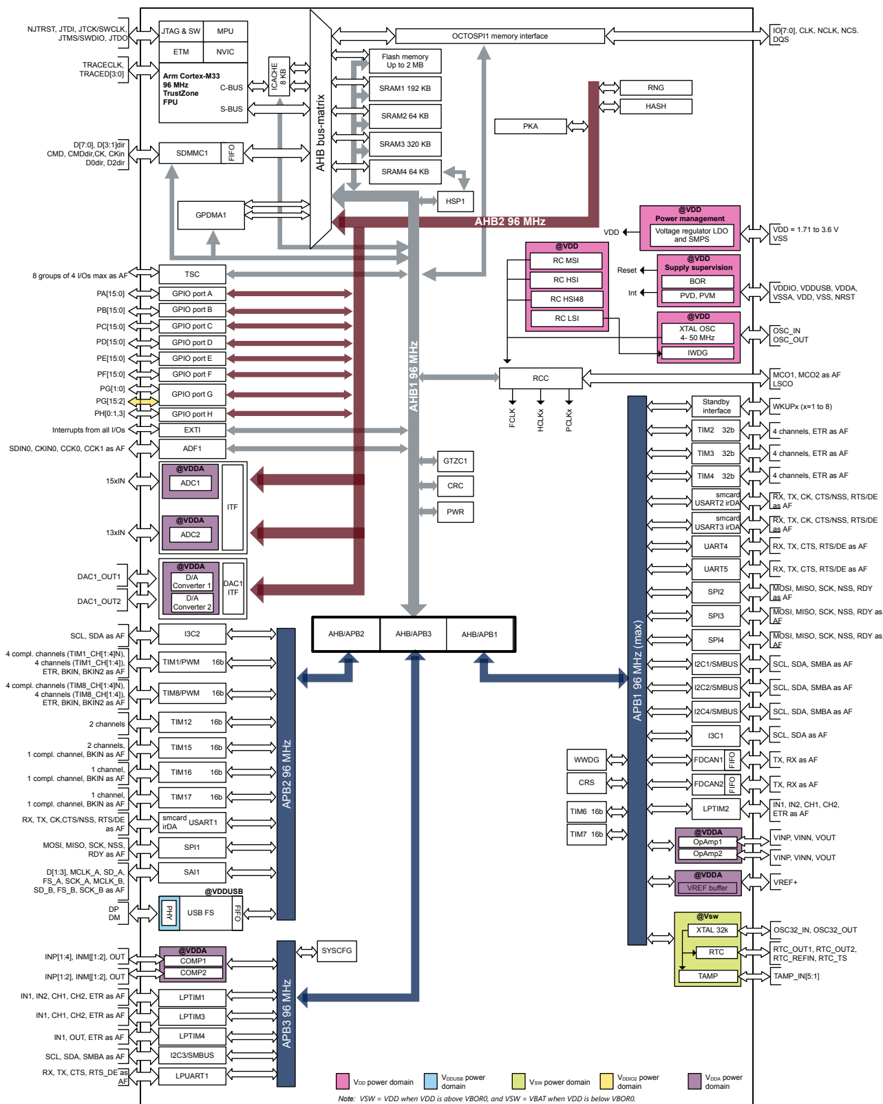
Figure 1. STM32U3B5xx block diagram
