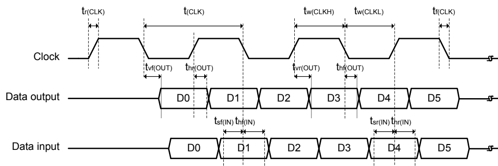
Figure 49. OCTOSPI timing diagram - DDR mode
