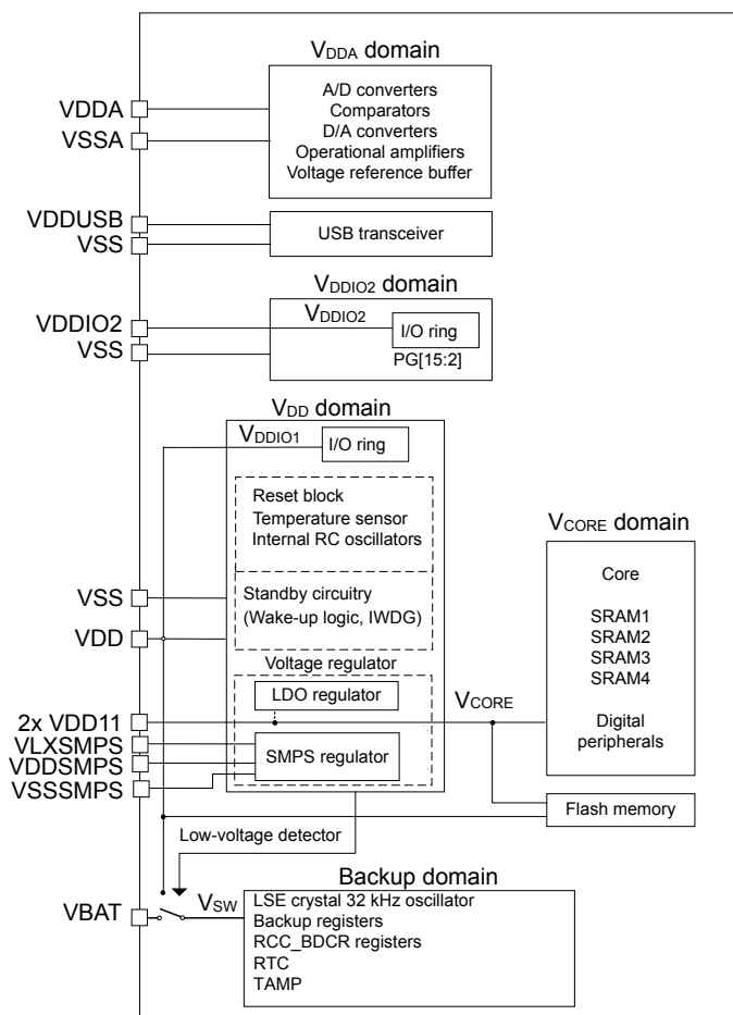
Figure 3. STM32U3B5xxxQ power supply overview (with SMPS)
