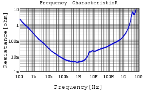
GRM31CR71C475KA01 R DCOV,25degC
