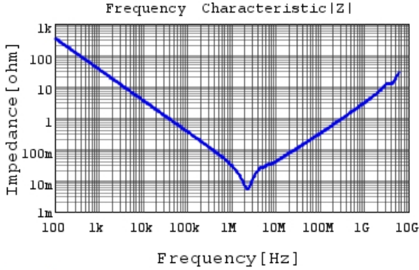
GRM31CR71C475KA01 |Z| DCOV,25degC
