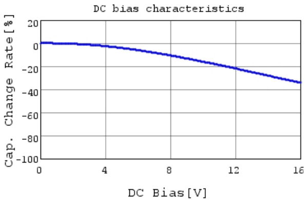
GRM31CR71C475KA01 C-DC bias capchange, 25.0c
