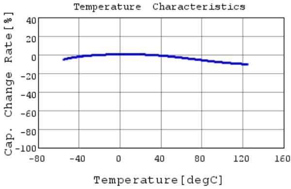
GRM31CR71C475KA01 C-Temp. capchange, DC0.0V,
