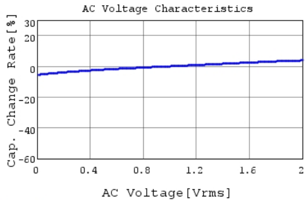
GRM31CR71C475KA01 C-AC Voltage capchange, D
