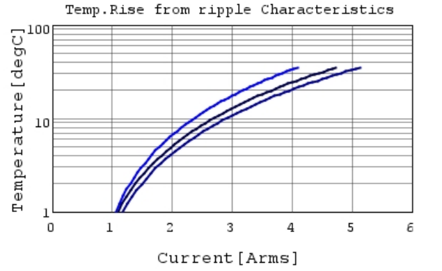
GRM31CR71C475KA01 Temp.rise — 100kHz
