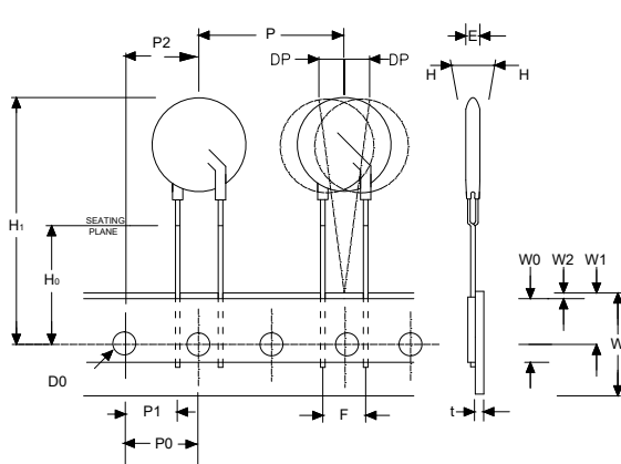
In-line Leads L3
