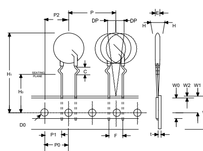
Inner Crimped Leads L5
