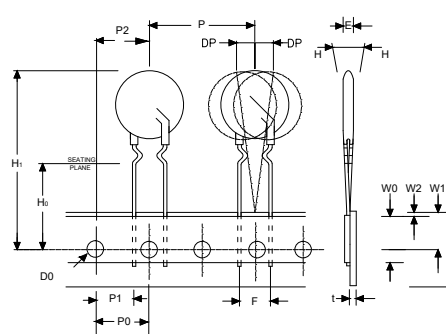
Inner Crimped Leads L5
