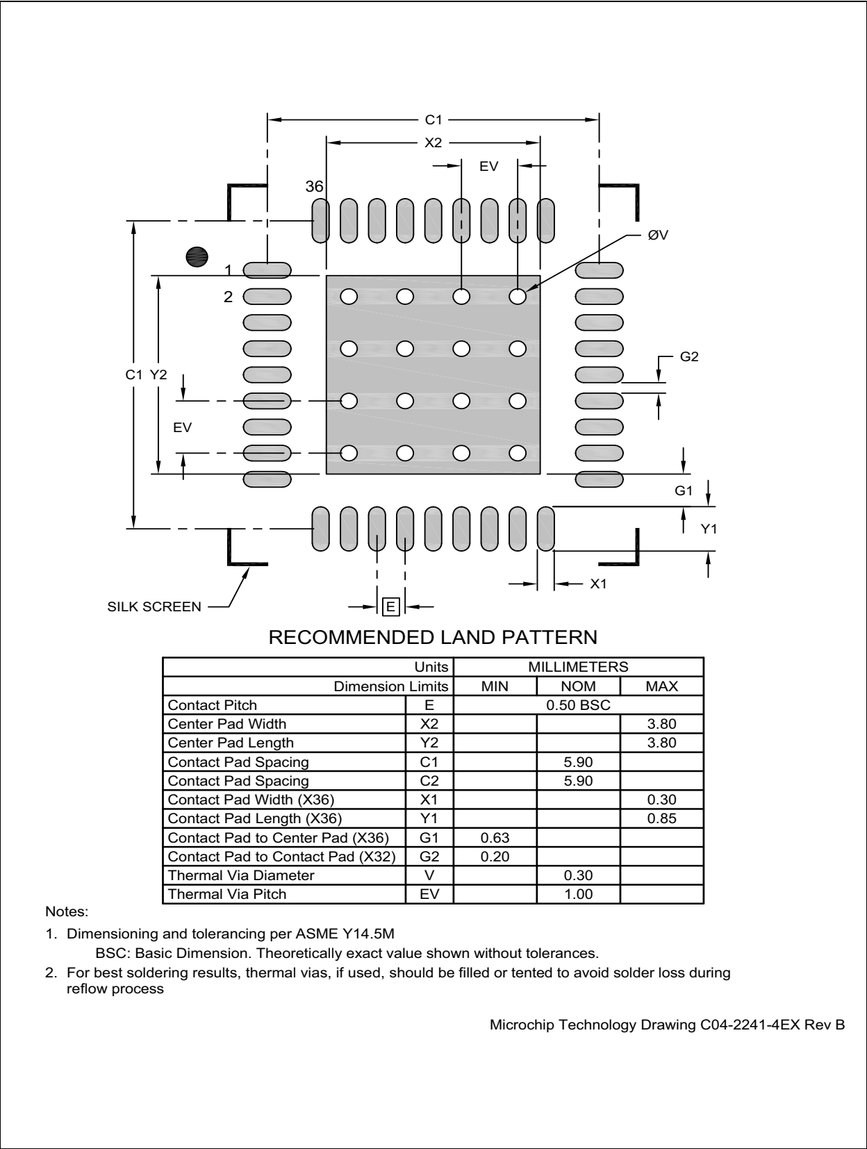
FIGURE 10-3: 36-QFN DIMPLE PACKAGE (LAND PATTERN)
