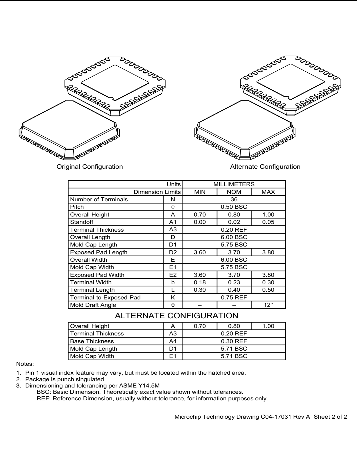
FIGURE 10-5: 36-QFN STANDARD PACKAGE (DIMENSIONS)
