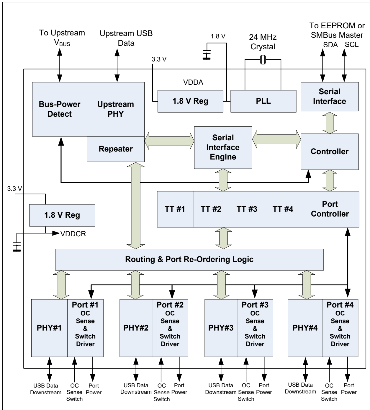
FIGURE 5-1: USB82514 BLOCK DIAGRAM
