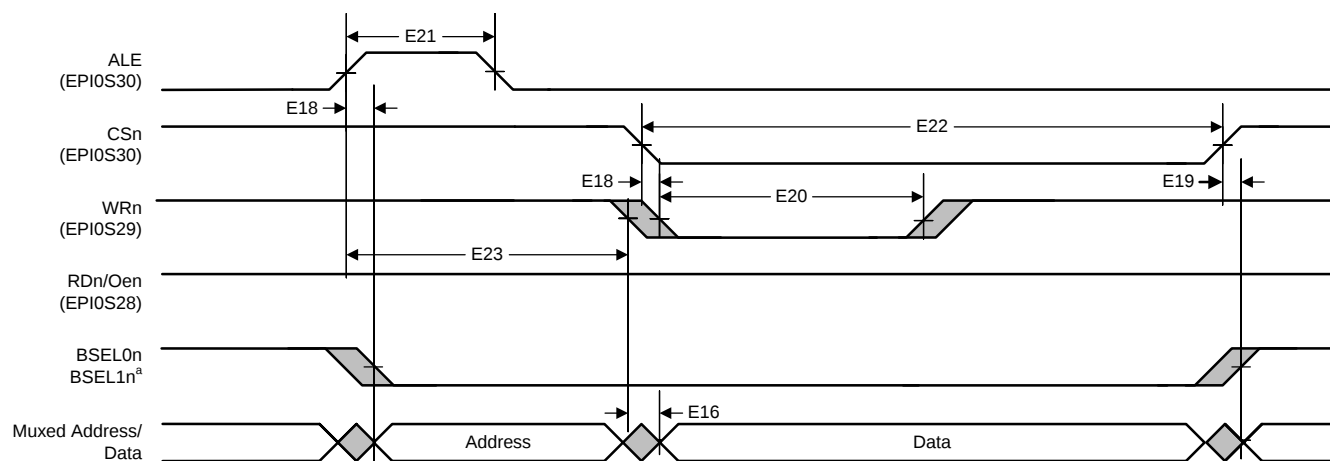
Figure 5-22. Host-Bus 8/16 Mode Asynchronous Muxed Write Timing
