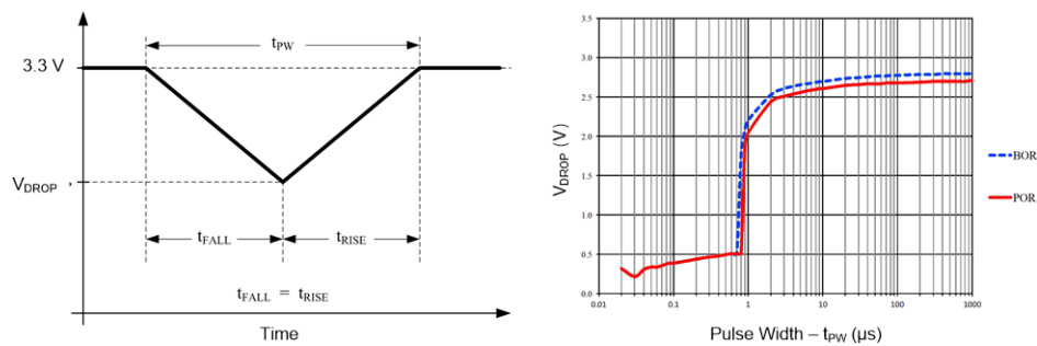
Figure 5-5. POR-BOR V_{DD} Glitch Response
