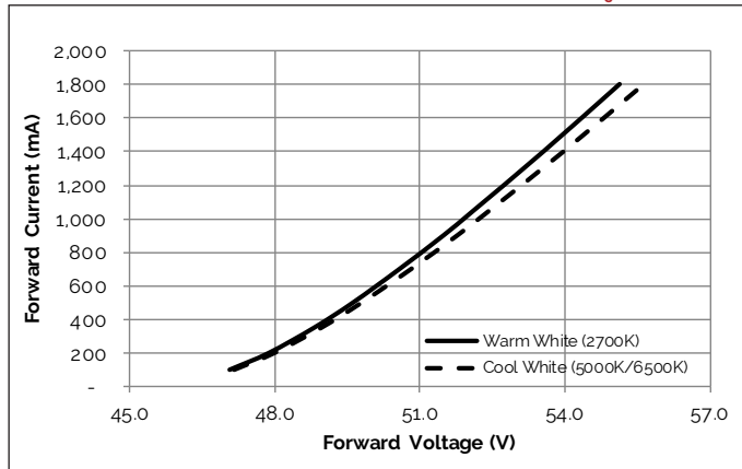
Figure 1: Forward Voltage vs. Forward Current, T_c = 25^\circ\text{C}
