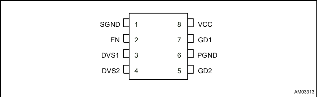
Figure 2. Pin configuration
