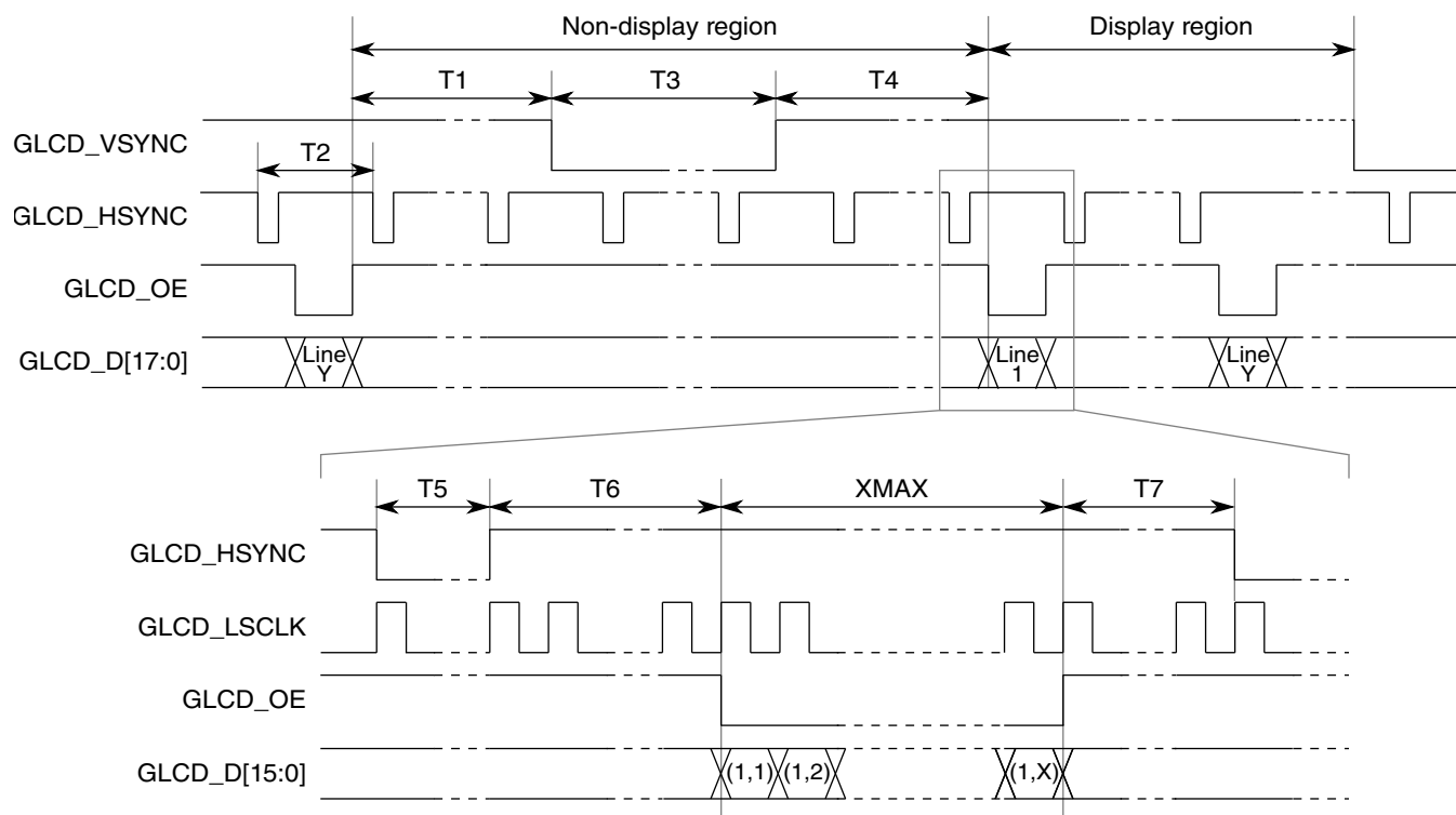
Figure 46. 4/8/12/16/18 Bit/Pixel TFT Color Mode Panel Timing
