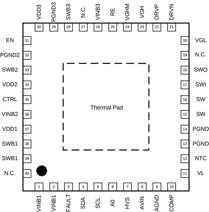
Figure 2. Pin Configuration
