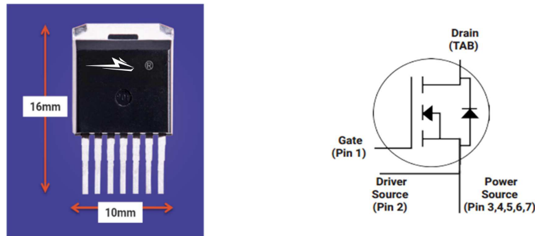
Figure 3: C2M1000170J SiC MOSFET in a TO-263-7 package
