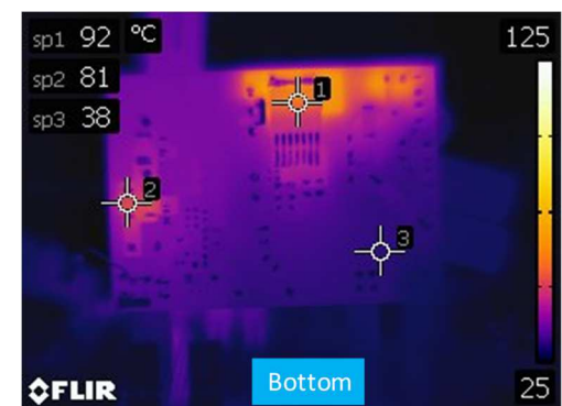
Figure 21: Thermal image of bottom layer at 1.2kVDC input and full load
