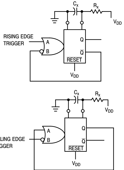
Figure 8. Non-Retriggerable Monostables Circuitry
