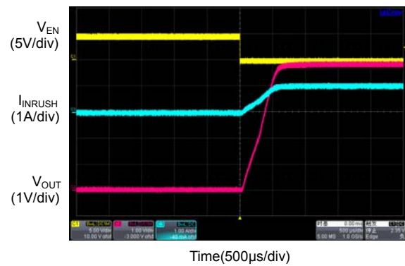
Figure 13. Output Turn ON and Rise Time ( C_{IN}=1.0\mu F , C_{OUT}=1.0\mu F , R_L=5.0\Omega )
