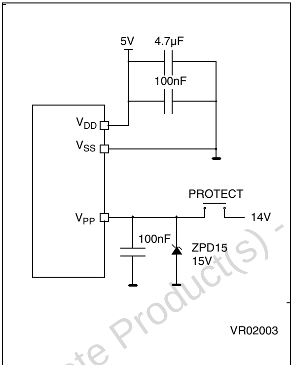
Figure 79. Programming Circuit
