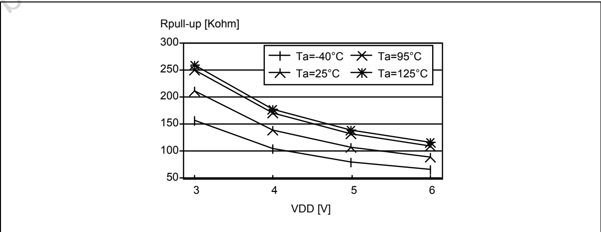
Figure 71. Typical R_{\text{pull-up}} vs. V_{\text{DD}} with V_{\text{IN}}=V_{\text{SS}}
