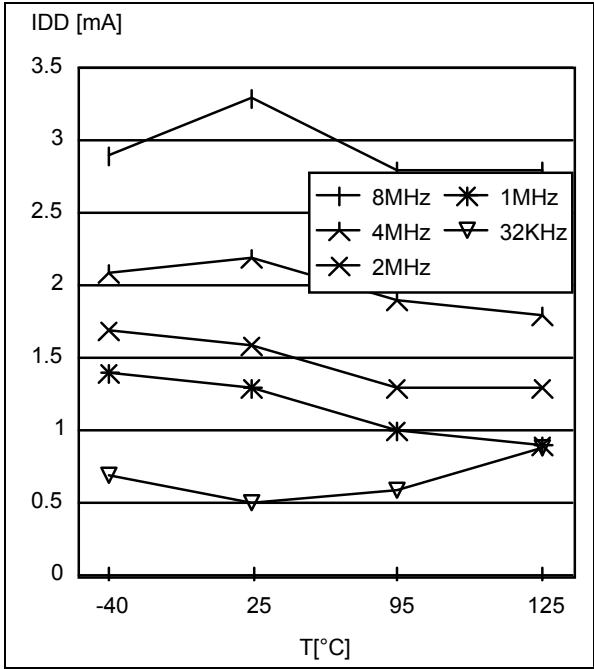
Figure 43. Typical I_{DD} in RUN vs. Temperature ( V_{DD} = 5\text{V} )
