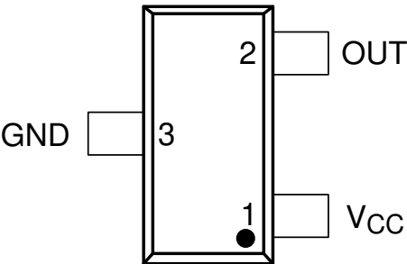
Figure 5-1. DBZ Package 3-Pin SOT-23 Top View
