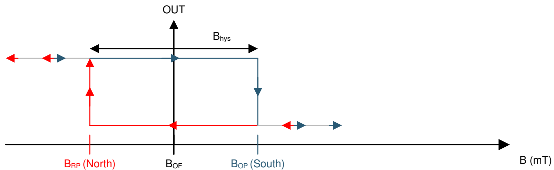
Figure 7-2. DRV5013 — B_{OP} > 0
