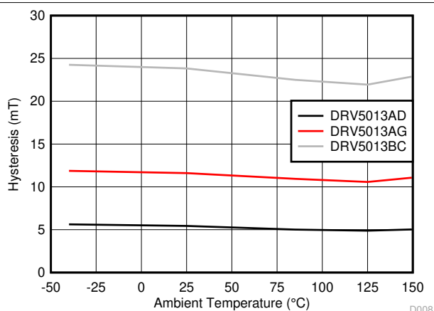
Figure 6-8. Hysteresis vs Temperature
