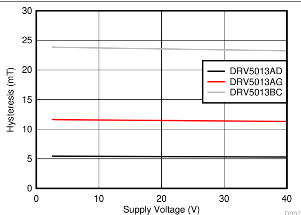
Figure 6-7. Hysteresis vs V_{CC}
